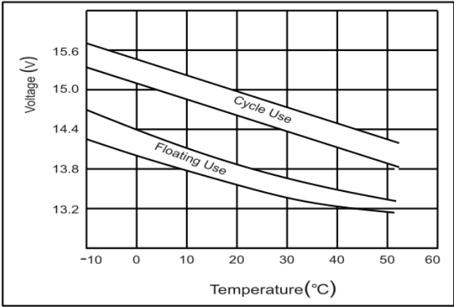
The relationship between charging voltage and temperature
