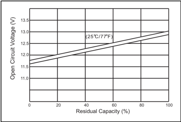
Relationship between OCV and capacity(25°C)
